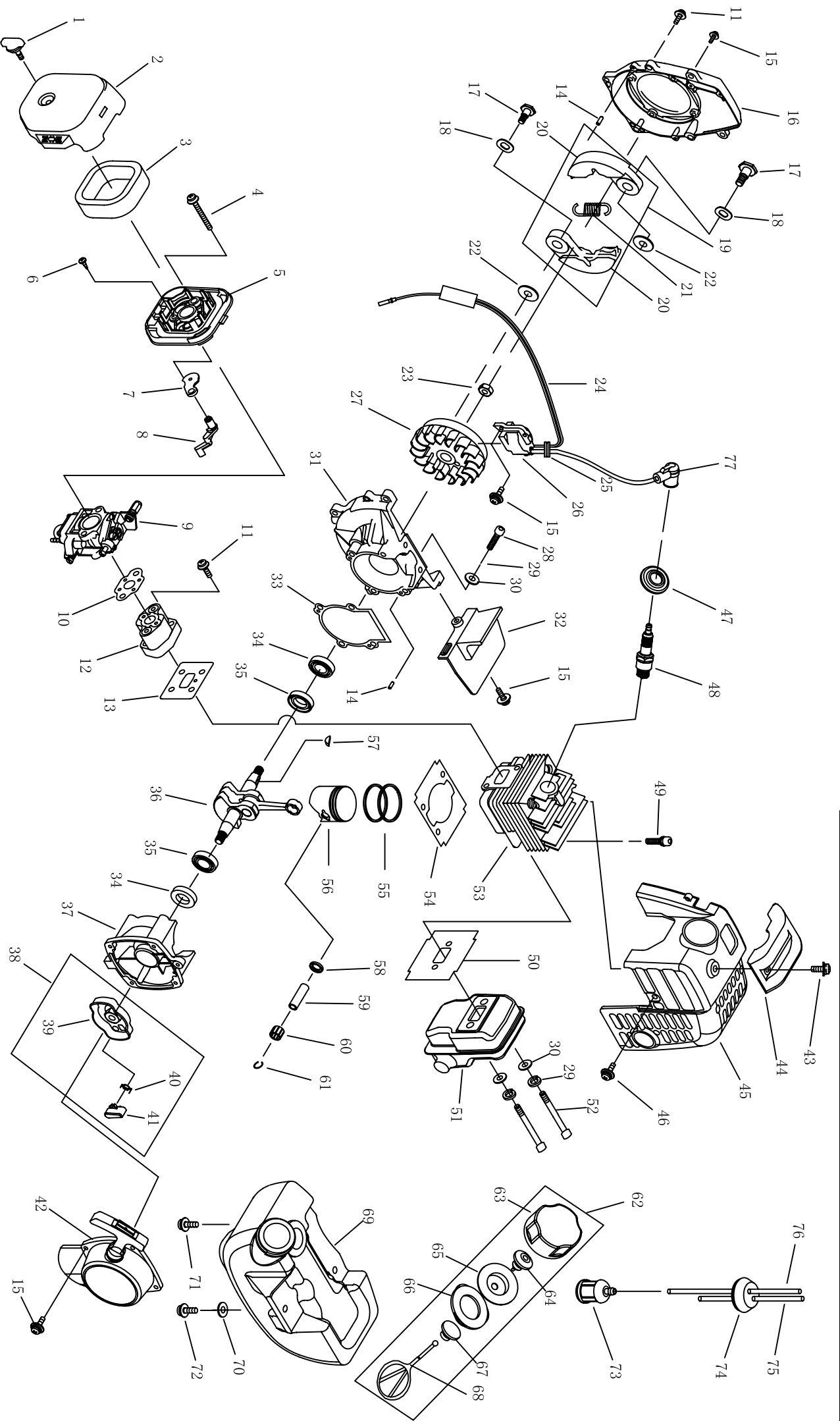
FIG. 1: 1E34F-CE GASLINE ENGINE
